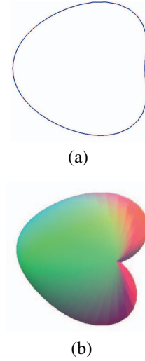
Figure 4. The bean shaped models
