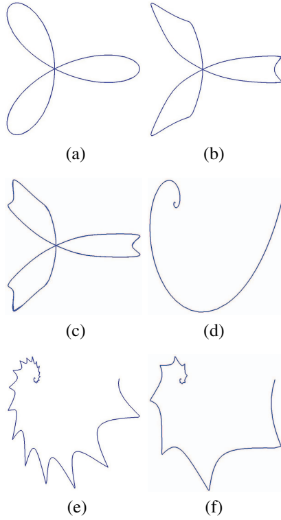
Figure 3. Geilis curves modified by f(\theta) . f(\theta) = \cos(4\theta) , m = 4 , n_1 = n_2 = n_3 = 100 , m = 5 , n_1 = n_2 = n_3 = 5 f(\theta) = \exp(0.5\theta) , m = 4 , n_1 = n_2 = n_3 = 100 , m = 2 , n_1 = n_2 = n_3 = 100
