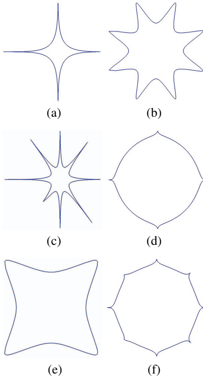
Figure 2. Examples of various abstract shapes. (a) and (c) n_1 = n_2 = n_3 = \frac{1}{3} , (b) and (e) n_1 = 10, n_2 = n_3 = 20 , (d) and (f) n_1 = 3, n_2 = n_3 = \frac{1}{3} .
