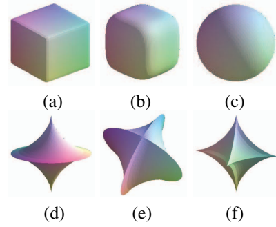
Figure 1. Superquadric shapes varying \epsilon_1, \epsilon_2 . (a) \epsilon_1 = \epsilon_2 = 0.1 , (b) \epsilon_1 = \epsilon_2 = 0.5 , (c) \epsilon_1 = \epsilon_2 = 1 , (d) \epsilon_1 = 3, \epsilon_2 = 1 , (e) \epsilon_1 = 1, \epsilon_2 = 3 , (f) \epsilon_1 = \epsilon_2 = 3 .
