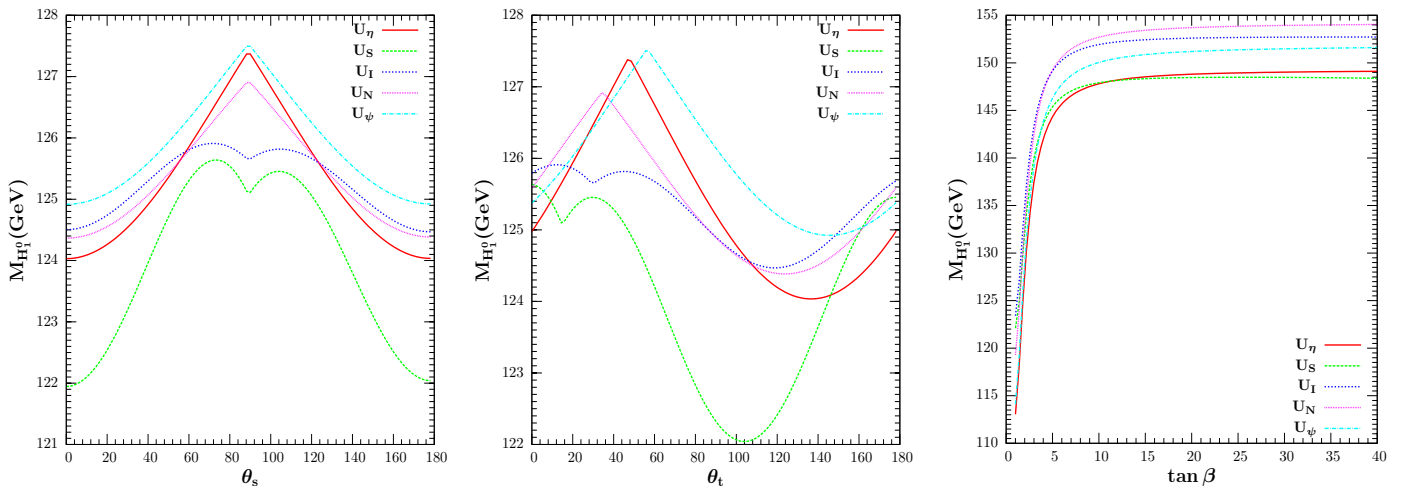
FIG. 2. Mass of the lightest neutral Higgs boson as a function of \theta_s (the phase of the new singlet S ), \theta_t (the phase of the soft coupling A_t ), and \tan\beta for the CP-violating versions of U(1)_\eta , U(1)_S , U(1)_I , U(1)_N and U(1)_\psi models.
