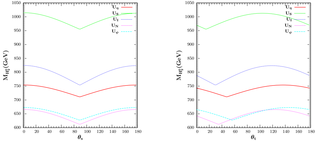
FIG. 4. M_{H_2^0} as a function of \theta_s (the phase of the new singlet S ) and \theta_t (the phase of the soft coupling A_t ) for the CP-violating versions of the U(1)_\eta , U(1)_S , U(1)_I , U(1)_N and U(1)_\psi models.
