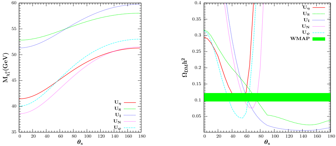
FIG. 1. Mass of the lightest neutralino and the relic density as functions of \theta_s (the phase of the new singlet S ) for the CP-violating versions of U(1)_\eta , U(1)_S , U(1)_I , U(1)_N and U(1)_\psi models. The green band indicates the experimentally allowed region.
