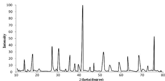
Fig. 1. Powder XRD pattern of \text{Co}_3\text{V}_2\text{O}_8 .
