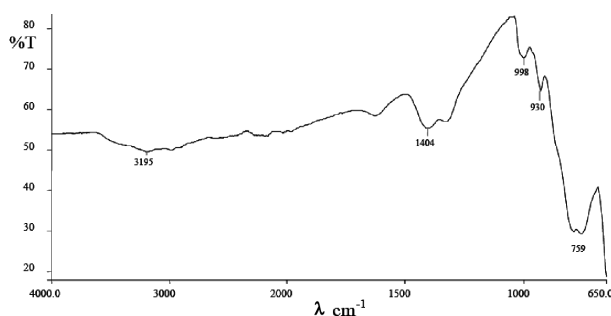
Fig. 2. FTIR spectrum of \text{Co}_3\text{V}_2\text{O}_8 .
