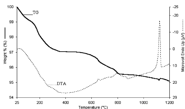
Fig. 3. TG/DTA curves of pure \text{Co}_3\text{V}_2\text{O}_8 .
