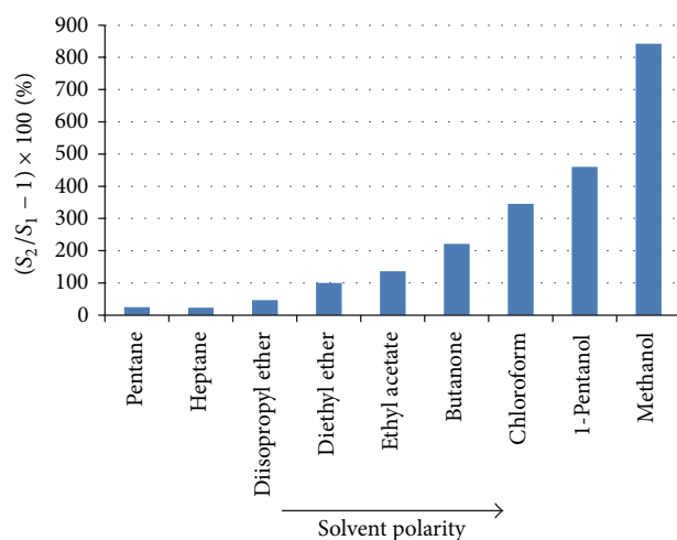
FIGURE 8: The ratio S_2/S_1 - 1 calculated as the increase in MWCNT ( \text{BuNH}_2 ) sensitivity with respect to sensitivity of pure MWCNT in trend of increased VOC polarity defined by total Hildebrand solubility parameter.
