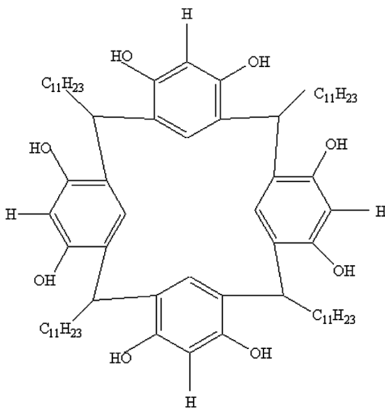
Figure 3. The Chemical structure of Calix[4]arene.
