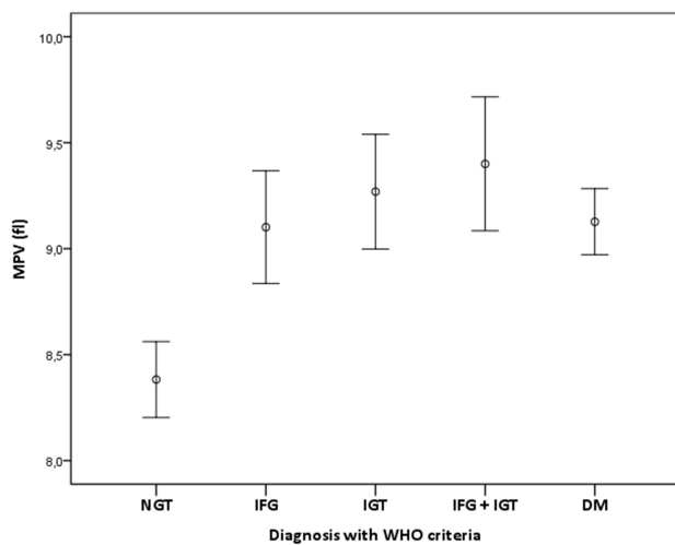
Figure 2. The distribution of mean platelet volume (MPV) levels among normal glucose tolerance (NGT), impaired fasting glucose (IFG), impaired glucose tolerance (IGT), IFG+IGT, diabetes mellitus (DM) individuals diagnosed with World Health Organization (WHO) criteria.
