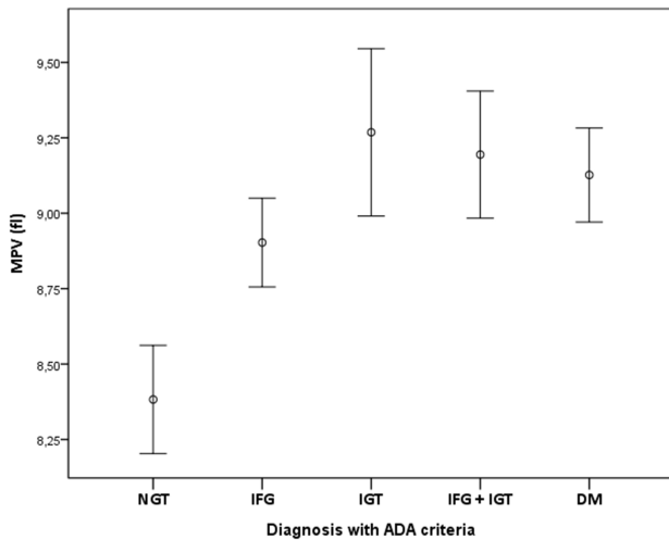
Figure 1. The distribution of mean platelet volume (MPV) levels among normal glucose tolerance (NGT), impaired fasting glucose (IFG), impaired glucose tolerance (IGT), IFG+IGT, diabetes mellitus (DM) individuals diagnosed with American Diabetes Association (ADA) criteria.
