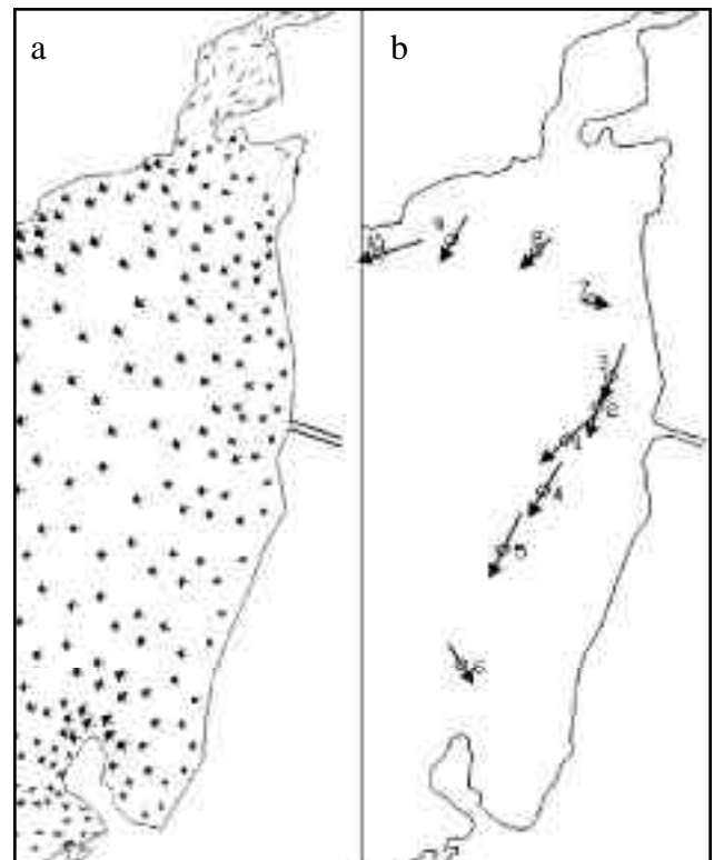
Figure 5 a. Calculated velocity vectors ( H_t = 0.60 \text{ m} , T_{\text{tide}} = 6 \text{ h} ) b. Measured velocity vector
