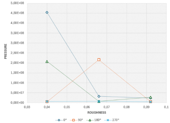
Fig. 4. Pressure vs. roughness and angle
