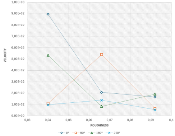
Fig. 9. Velocity vs. roughness and angle
