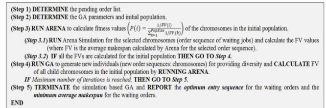
Figure 2. Pseudo Code used for scheduling by GA aided Arena simulation.
