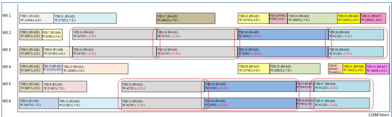
Figure 5. Gantt chart of the schedule with Arena without using GA (order number has priority).
