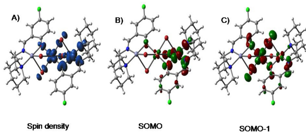
Figure 10. (A). Graphical representation of the spin density (contour 0.004 \text{ e } \text{\AA}^{-3} ) at the ground-state (high-spin) configuration of compound 5 . (B, C) Pictorial representation of the SOMO involving the d_{x^2-y^2} orbitals of \text{Cu}^{\text{II}} in compound 5 .
