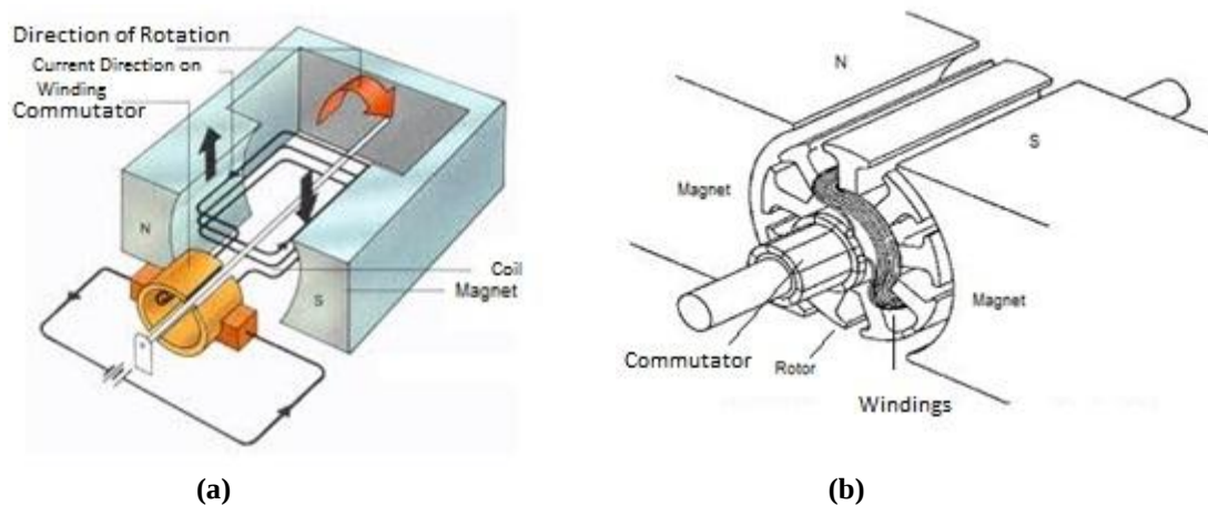
Fig.1.2: (a) Single winding, (b) Multiple winding brush DC motor [3].
