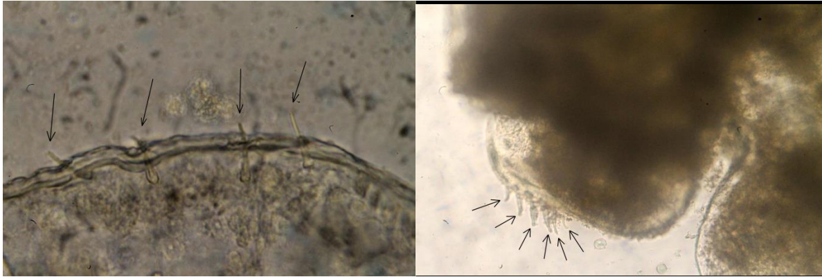
Figure 14: Ceratothoa parallela (♀): Hooks on medial of pleopod peduncle.
