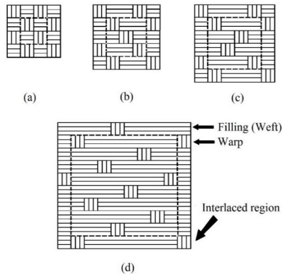
Figure 1. Examples of woven fabric patterns: (a) plain weave ( ng=2 ); (b) left twill \frac{1}{2} ( ng=3 ); (c) four-harness satin (crowfoot) ( ng=4 ); (d) eight-harness satin ( ng=8 ) [1]
