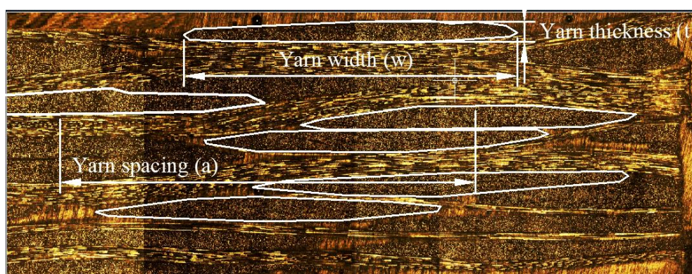
Figure 6. Representative cross-sectional view of glass woven fabric epoxy laminate
