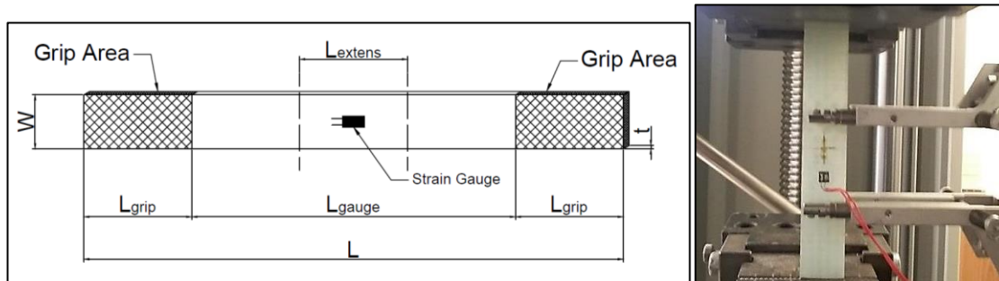
Figure 4. Schematic drawing and a photograph of a composite tensile test specimen mounted on the testing machine.
