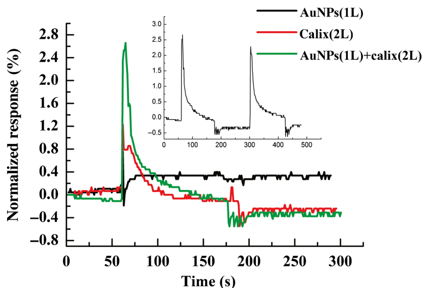
Figure 4. Kinetic gas response for the AuNPs monolayer, calix bilayers and their hybrid film obtained using SPR method under exposure to saturated vapour of chloroform. Inset: the kinetic response of the hybrid film obtained during two consecutive exposures of saturated vapour of chloroform.
