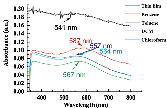
Figure 3. The UV–visible spectra of the unexposed hybrid film and the thin film under exposure to saturated benzene, toluene, DCM and chloroform vapours.
