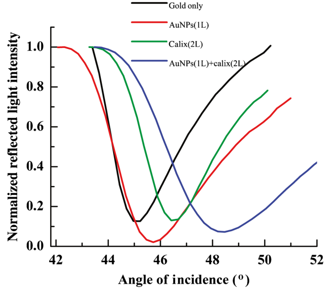
Figure 2. SPR curves of 1 layer of AuNPs, 2 layers of calixarene and the hybrid film with uncoated gold substrate.
