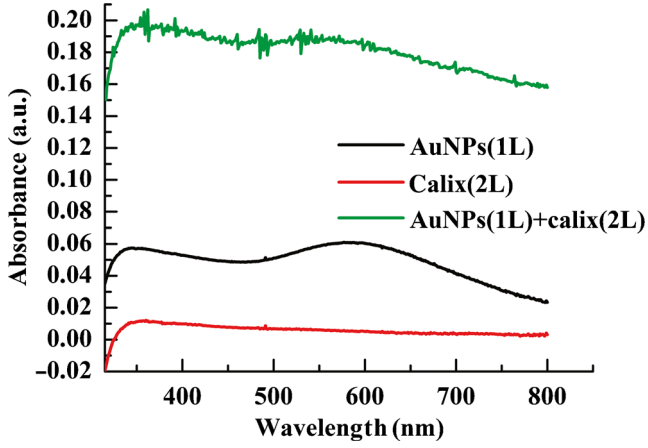
Figure 1. UV-visible spectra of thin films with 1 layer of AuNPs, 2 layers of calixarene and the hybrid film.
