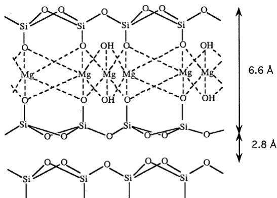
Fig. 7. Crystal structure of talc clay.
