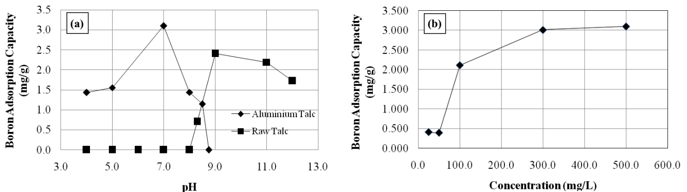
Fig. 2. (a) pH effect on boron adsorption of raw and modified talc and (b) Concentration effect on boron adsorption of modified talc.
