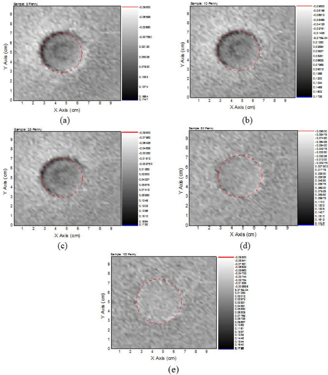
Figure 7. The graphs of tested coin samples a)5 Kurus, b)10 Kurus, c)25 Kurus, d)50 Kurus, e)1 Turkish Lira
